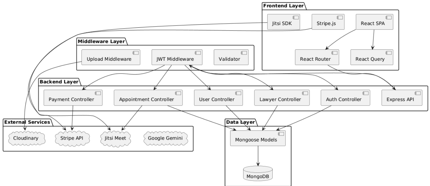
Figure 4.2: CounselDesk Component Architecture
