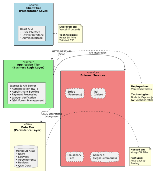
Figure 4.1: CounselDesk System Architecture
