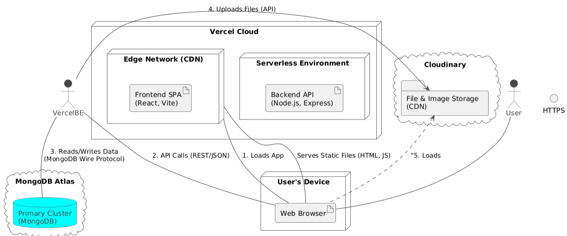
Figure 5.2: CounselDesk Deployment Architecture
