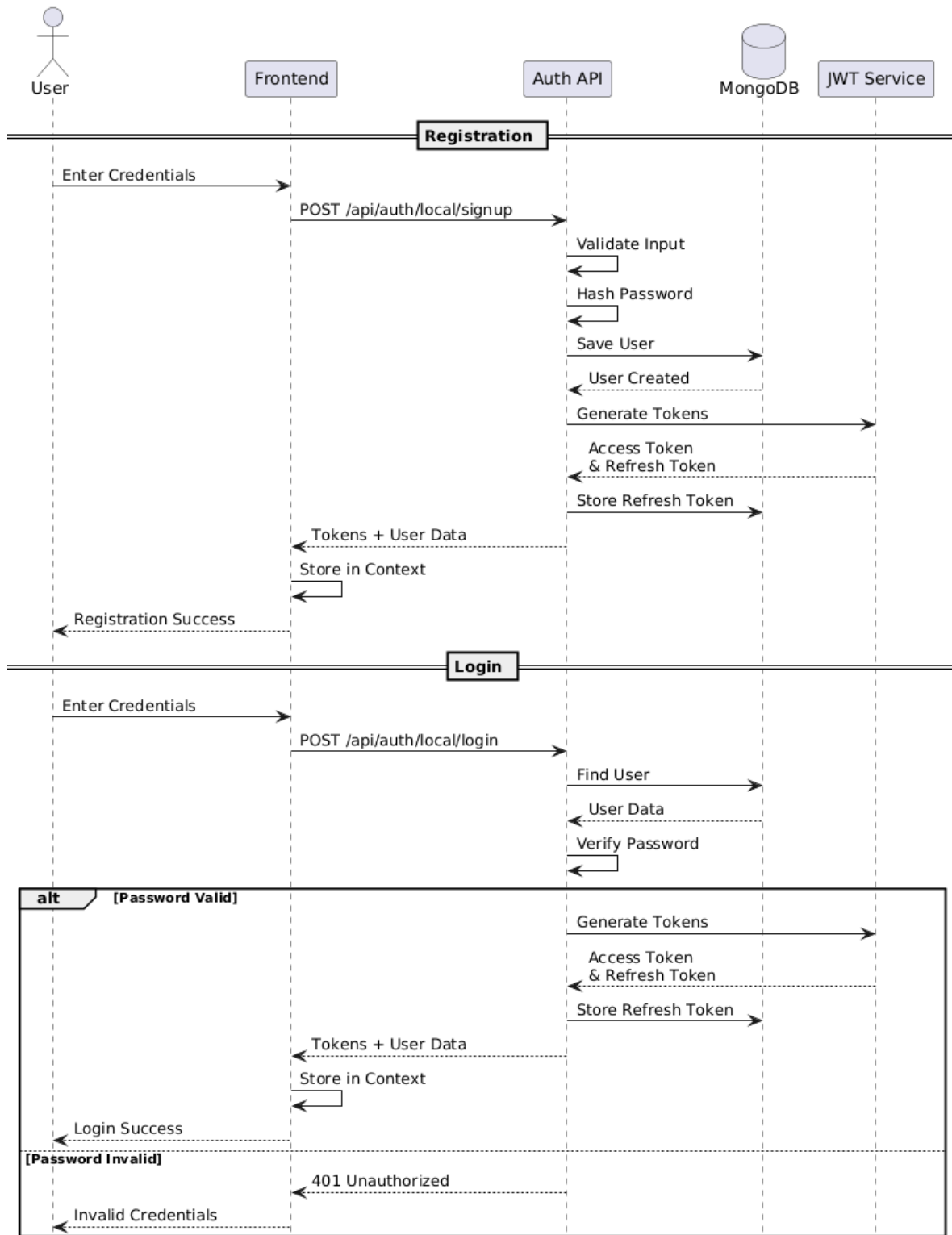
Figure 4.6: JWT Authentication Flow with refresh token
