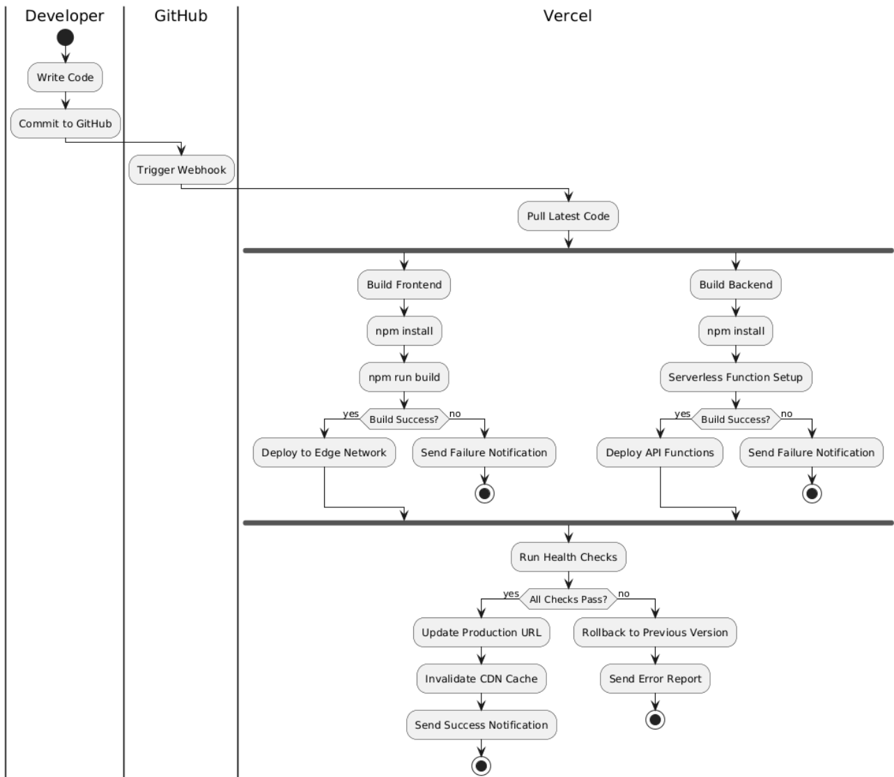
Figure 5.3: Automated Deployment Flow
