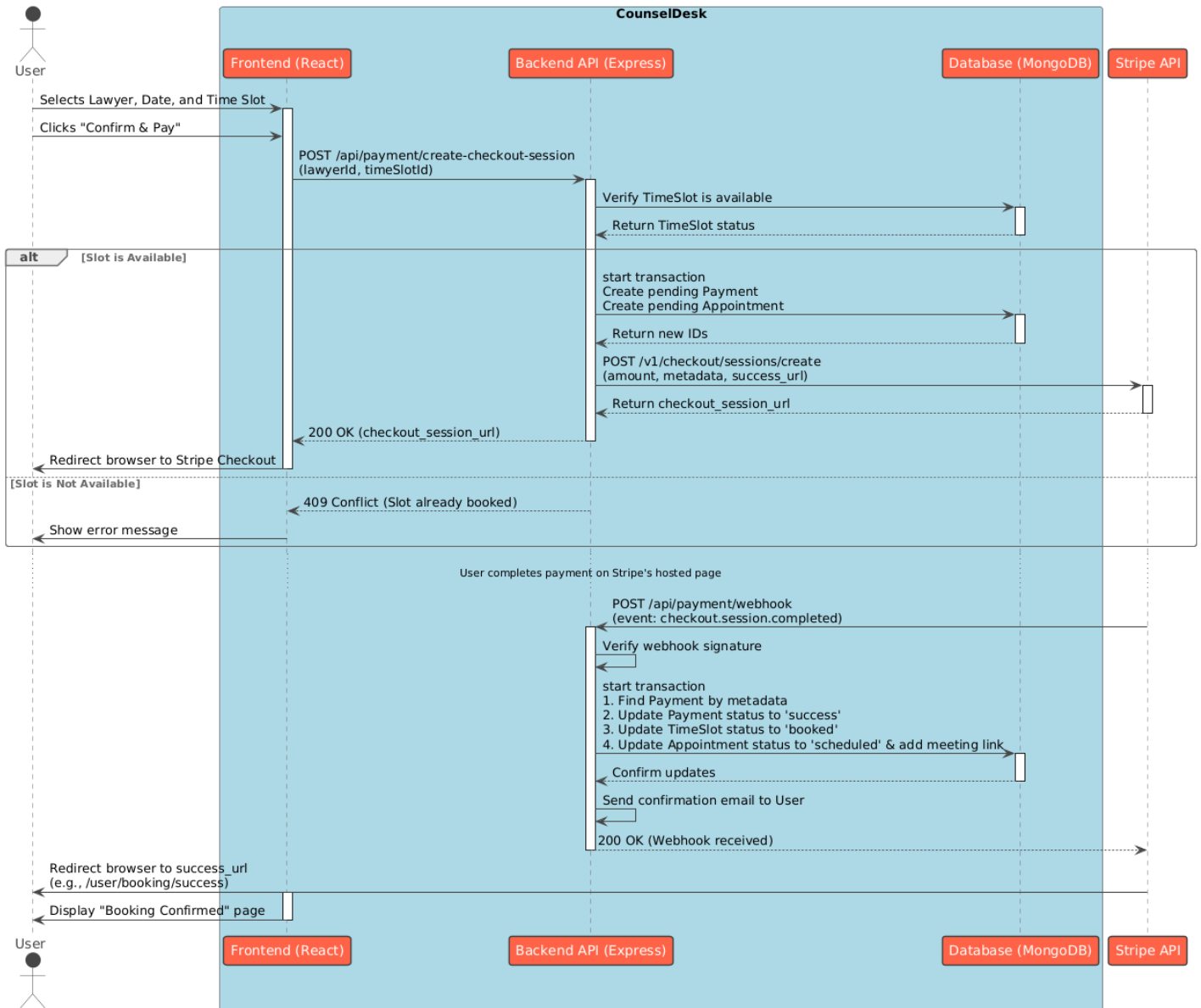
Figure 4.7: Appointment Booking Flow
