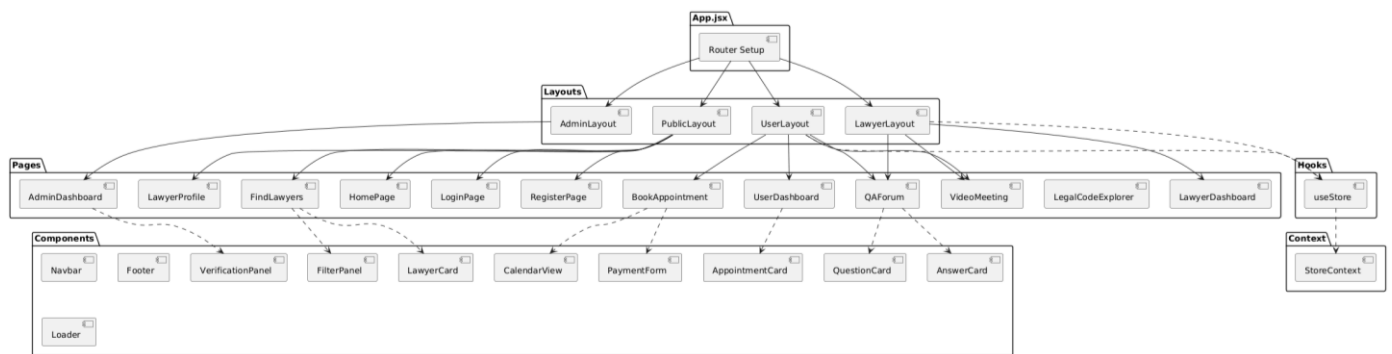
Figure 4.4: CounselDesk Frontend Component Hierarchy
