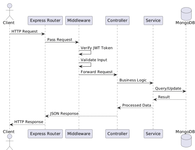
Figure 4.5: API Request Flow
